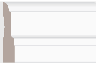
90431 5/8" x 3-1/4" 90431-96168C - 14'
