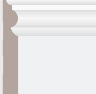
CR683 3/4" x 4-1/2" CR683-9U192C - 16'
