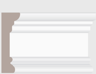
95000 1-3/16" x 3-3/4" 95000-96192C - 16'
